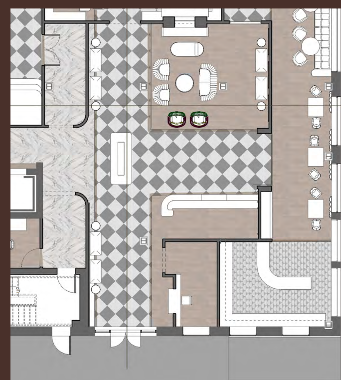
LOBBY & RECEPTION PLAN
